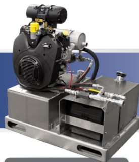
Kohler 32HP Gas Power Unit
